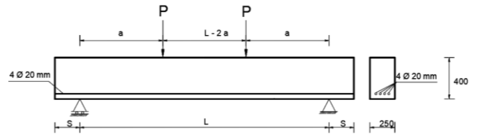
Fig. 11 Setup of the beam and cross-section details.
