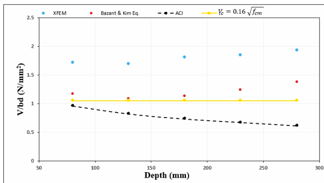
Fig. 8 Concrete strength versus beam depth relations for XFEM, Bažant and Kim Eq. and ACI code.
